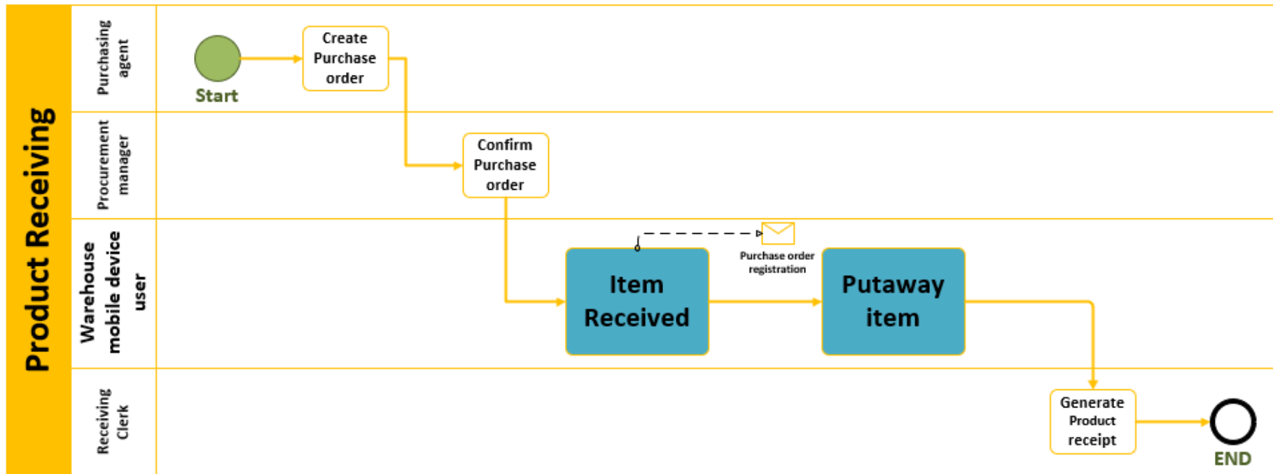
Figure 1 Process Flow Map (To-be)
